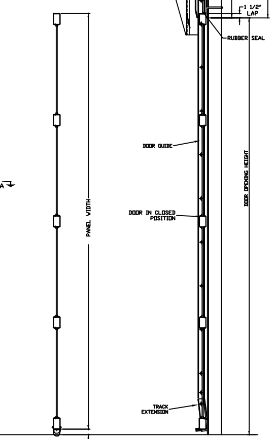
SECTION C-C
