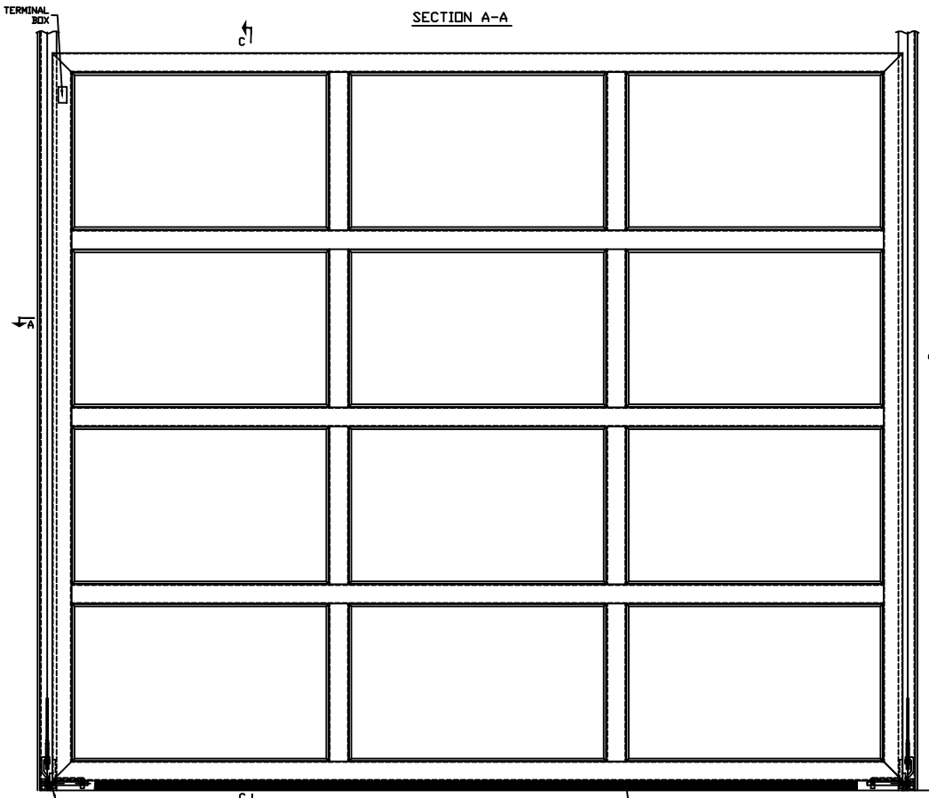
INTERIOR ELEVATION ONE LEAF TURNOVER DOOR
